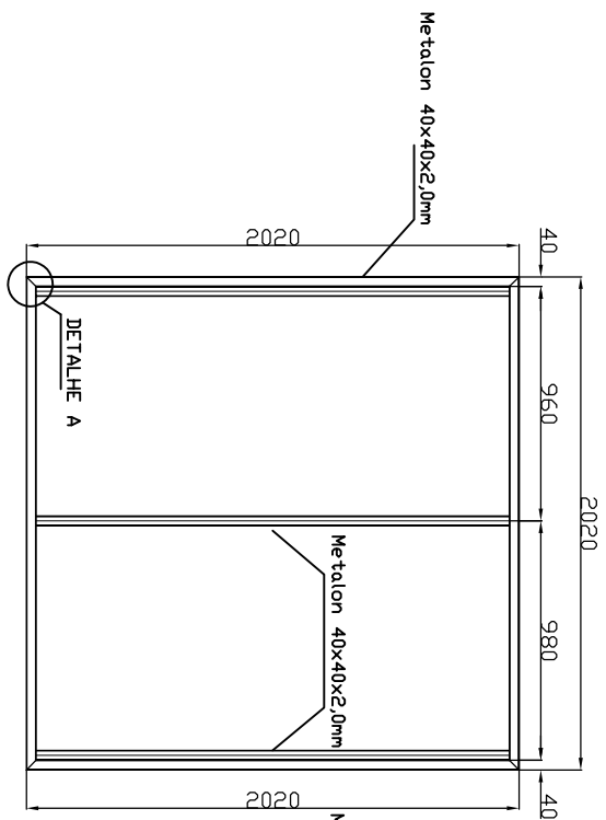
VISTA FRONTAL
